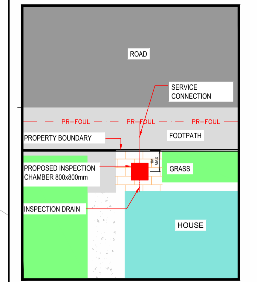
INSPECTION CHAMBER LOCATION TYPICAL DETAIL Scale at A1 1:100
